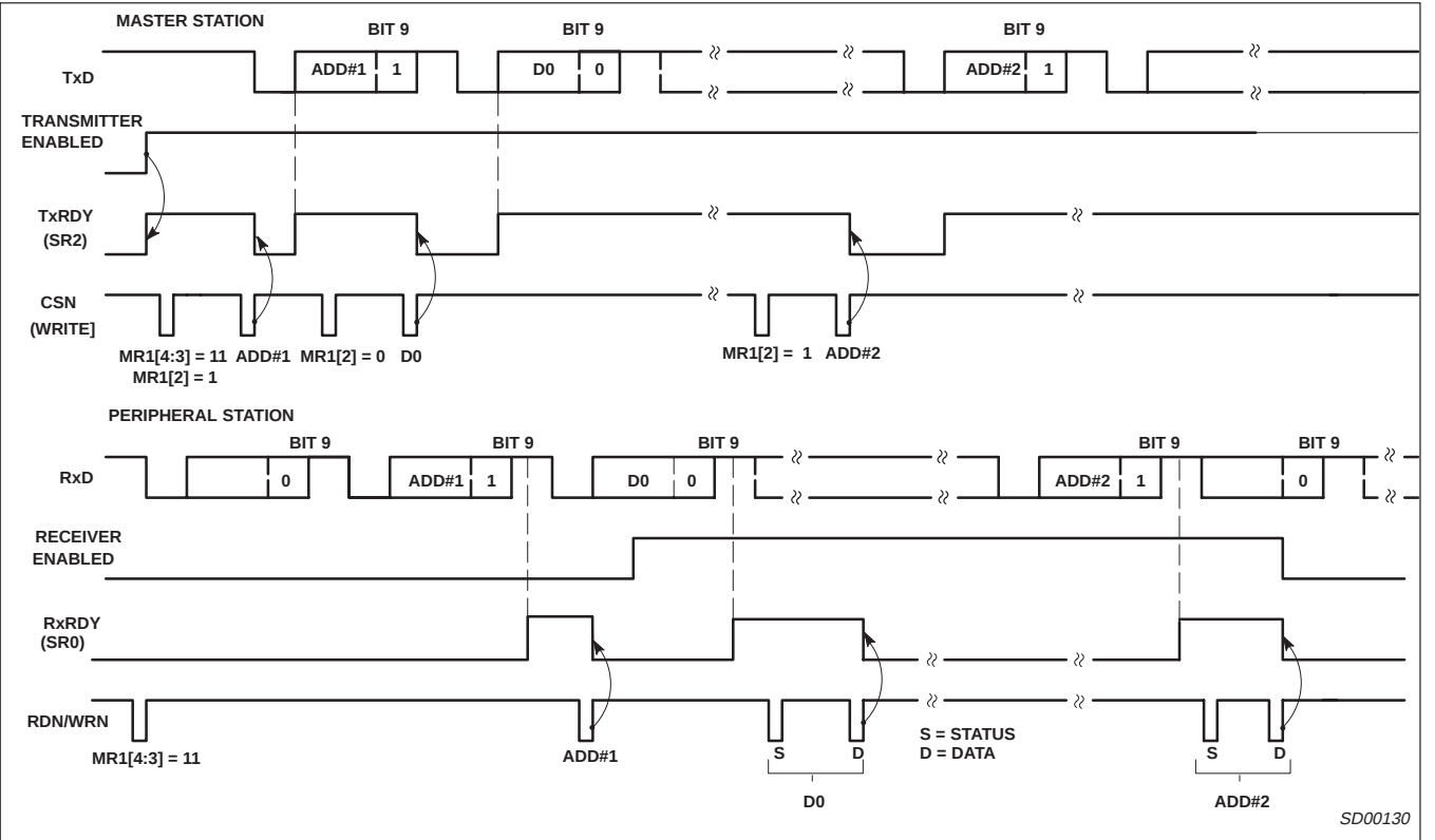
Figure 14. Wake-Up Mode
