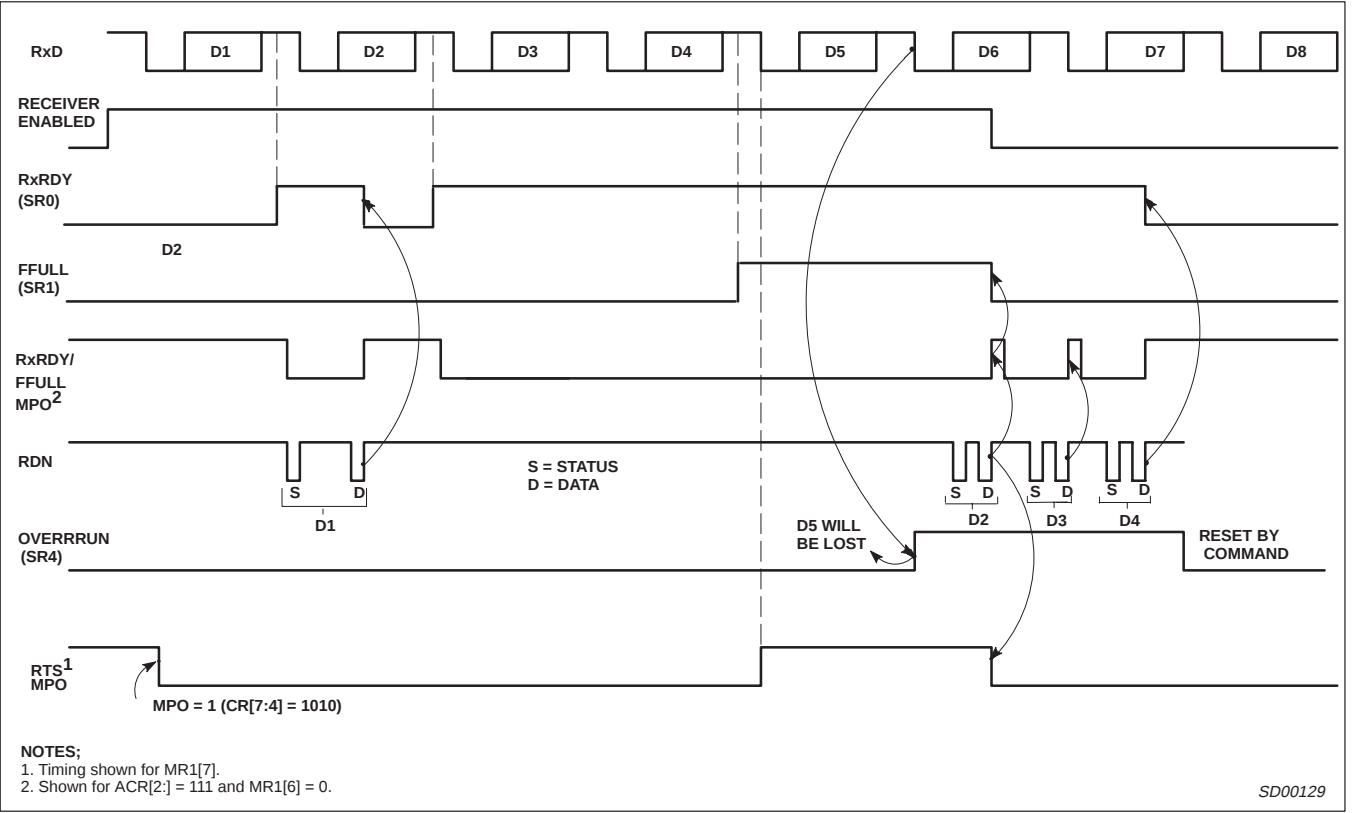
Figure 13. Receiver Timing
